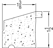
PVC-SN PVC Sill Nose
