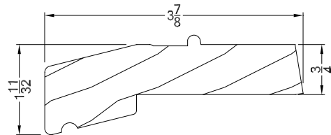
SS-H H Subsill
