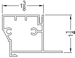
CBM 2" Clad Brickmould
