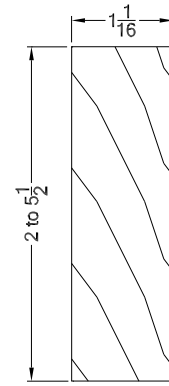
FCV Variable Width Flat Casing
