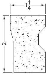
PVC-BM 2" PVC Brickmould
