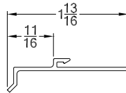
CSP Clad Sill Plate
