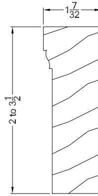
BMV Variable Width Brickmould
